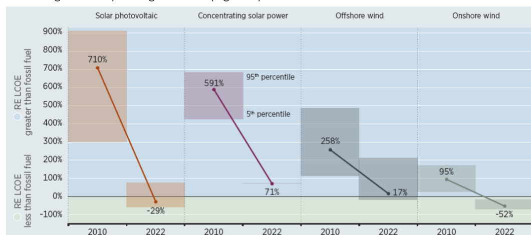
Figure 8: Change in competitiveness of solar and wind by country based on global weighted average LCOE, 2010-2022, IRENA 2023
