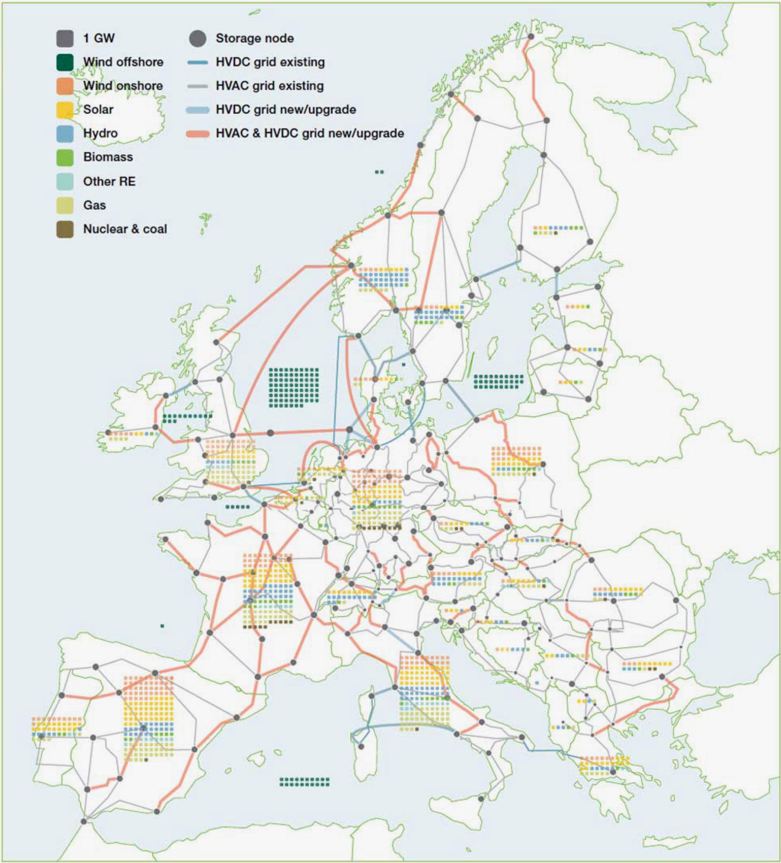
Figure 13 Overview of the future power system with 68% renewable electricity in 2030
